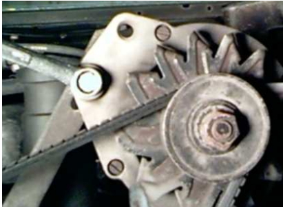
Manual Tensioning
